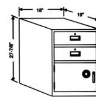
Model 622 is a sit-down height pedestal featuring two box drawers with No. 94 lock over a 1/4" frame, 1/2" door locker. The locker is equipped with 3 point boltwork, a group 2 combination lock and one adjustable shelf. Weight: 181 lbs.
