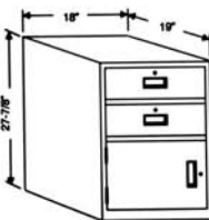
Model 604 is a sit-down height pedestal featuring two box drawers with No. 94 lock over one double pan door with No. 94 lock. The unit includes one adjustable shelf. Weight: 122 lbs.
