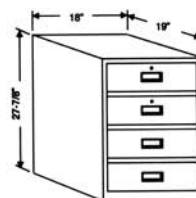
Model 608 is a sit-down height pedestal featuring four box drawers. The unit's top two drawers include a No. 94 lock. Weight: 158 lbs.
