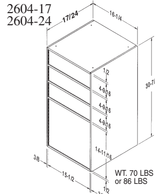
SINGLE WIDTH, (3) TELLER LOCKERS OVER (1) MANAGER CASH LOCKER, 16-1/4" W x 30-7/8" H x 17" D or 24" D
