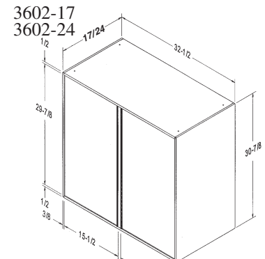
DOUBLE WIDTH, (2) MULTI-TASK LOCKERS, 32-1/2" W x 30-7/8" H x 17" D or 24" D
