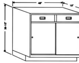
Model 267 is a 48" wide pedestal with two box drawers over two double pan sliding doors. The unit includes one adjustable shelf. Weight: 199 lbs.
