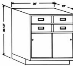
Model 251 features four box drawers over two double pan sliding doors. The unit includes one adjustable shelf. Weight: 207 lbs.
