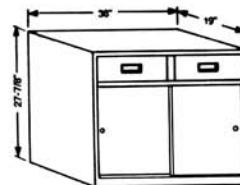
Model 641 is a sit-down height pedestal featuring two box drawers over two double pan sliding doors. The unit includes one adjustable shelf. Weight: 161 lbs.
