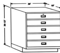
Model 229 features five full width drawers. The top drawer is equipped with a No. 94 lock. As a costed option, full width inserts and/or a ganglock is available. Weight: 291 lbs.
