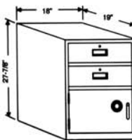
Model 620 is a sit-down height pedestal featuring two box drawers with No. 94 lock over a full 1/2" locker with a 1/4" door locker. The locker is equipped with 3 point boltwork, a group 2 combination lock and one adjustable shelf. Weight: 170 lbs.
