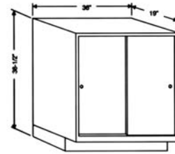
Model 231 features two double pan sliding doors and two adjustable shelves. Weight: 160 lbs.
