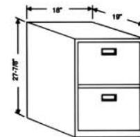
Model 609 is a sit-down height pedestal featuring two legal drawers w/HS. Weight: 124 lbs.
