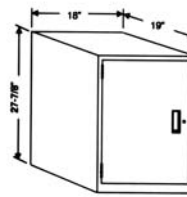
Model 602 is a sit-down height pedestal with a double pan door with No. 94 lock. The unit includes one adjustable shelf. Weight: 92 lbs.
