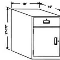
Model 603 is a sit-down height pedestal featuring one box drawer with No. 94 lock over a double pan door with No. 94 lock. The unit includes one adjustable shelf. Weight: 107 lbs.
